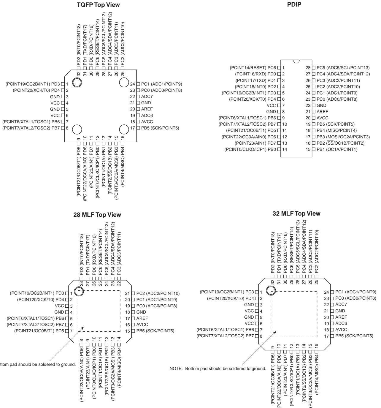
Figure 1-1. Pinout ATmega48/88/1682545LS
